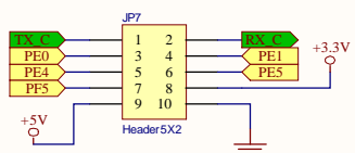
EXPANDER 2
