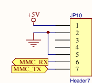
MICRO MMC
